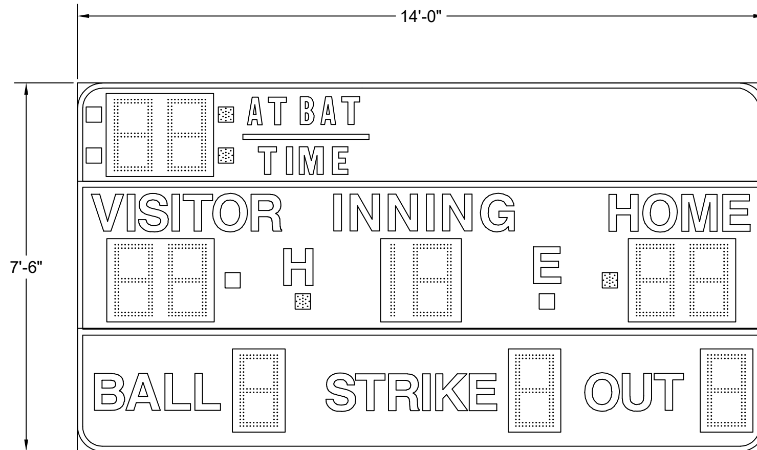
BA-7200MP-2 7'-0"L HANGER SPACING, STANDARD J BRACKET
