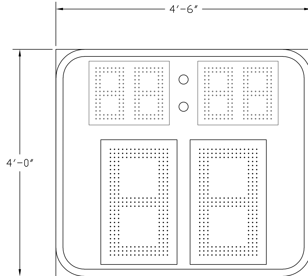
T-0448-06-DISPLAY-2 GAME CLOCK/PLAY CLOCK DISPLAY TOP: GAME CLOCK USING 12"H AMBER LED DIGITS BOTTOM: PLAY CLOCK USING 24"H AMBER LED DIGITS
