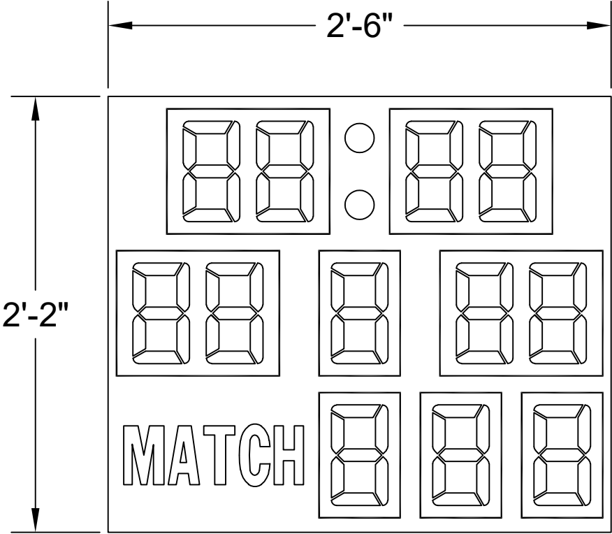
WR-1400-2S-4 FACE 1 SHOWN, FACE 2 TYPICAL
