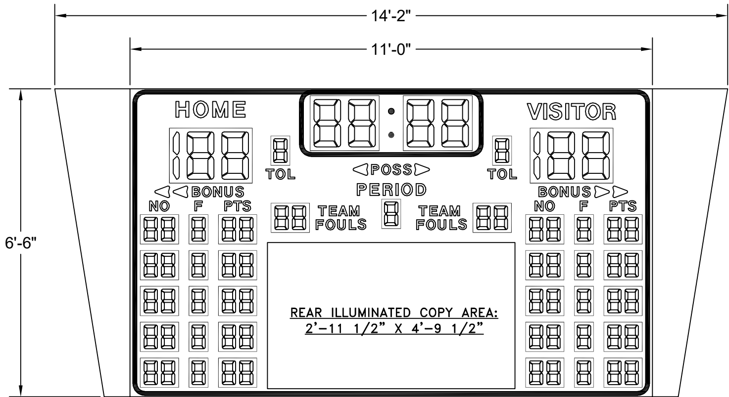
BB-1855B-4 FOUR-SIDED BASKETBALL SCOREBOARD SIDE 1 OF 4 SHOWN - ALL OTHERS TYPICAL
