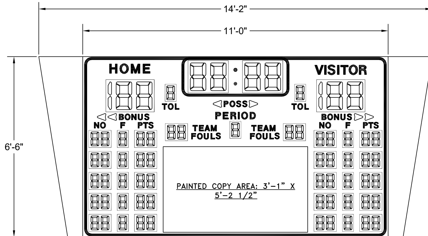
BB-1855A-4 FOUR-SIDED BASKETBALL SCOREBOARD FACE 1 OF 4 SHOWN - ALL OTHERS TYPICAL
