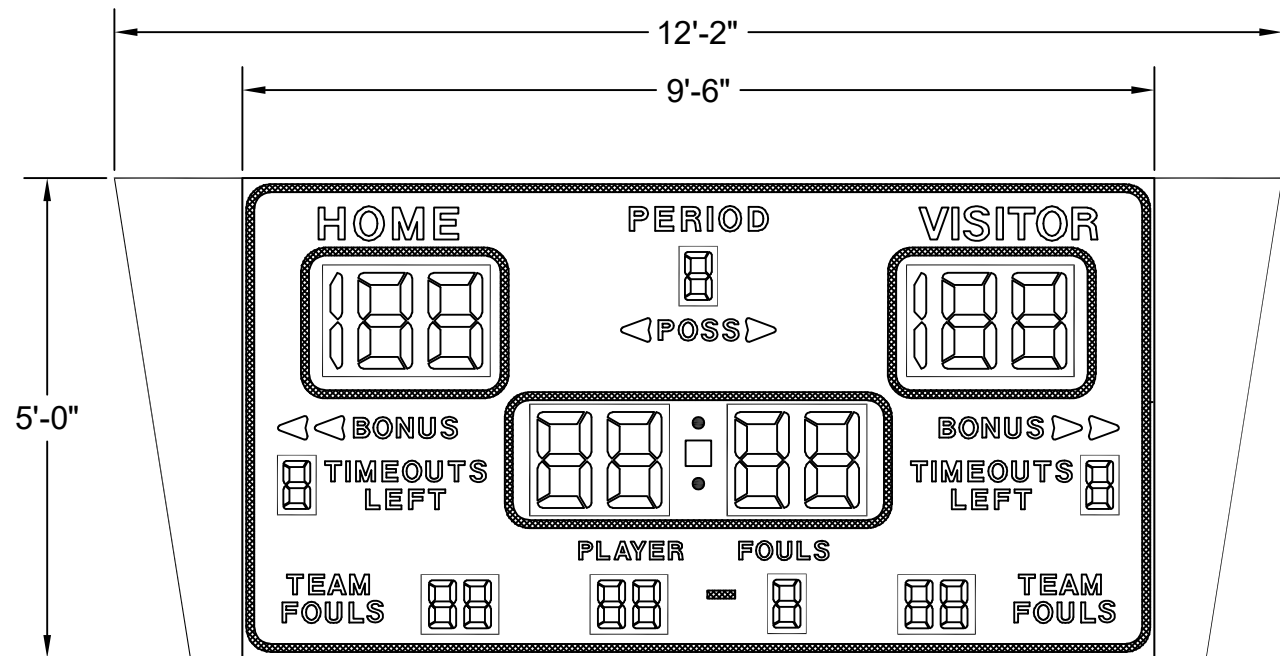
BB-1850-4 FOUR-SIDED BASKETBALL SCOREBOARD SIDE 1 OF 4 SHOWN - ALL OTHERS TYPICAL
