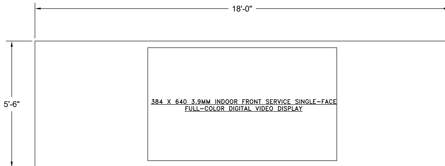
FACE VIEW SHOWN WITH 18'-0"L X 5'-6"H TRIM KIT, USING INDOOR FRAME
