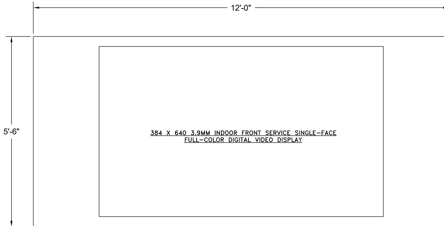
FACE VIEW SHOWN WITH 12'-0"L X 5'-6"H TRIM KIT, USING INDOOR FRAME
