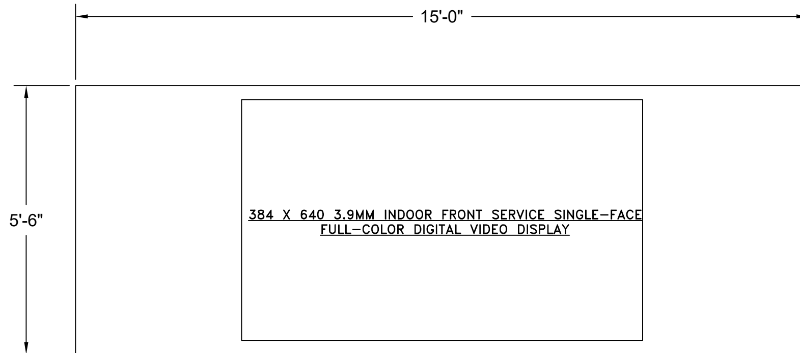
FACE VIEW SHOWN WITH 15'-0"L X 5'-6"H TRIM KIT, USING INDOOR FRAME
