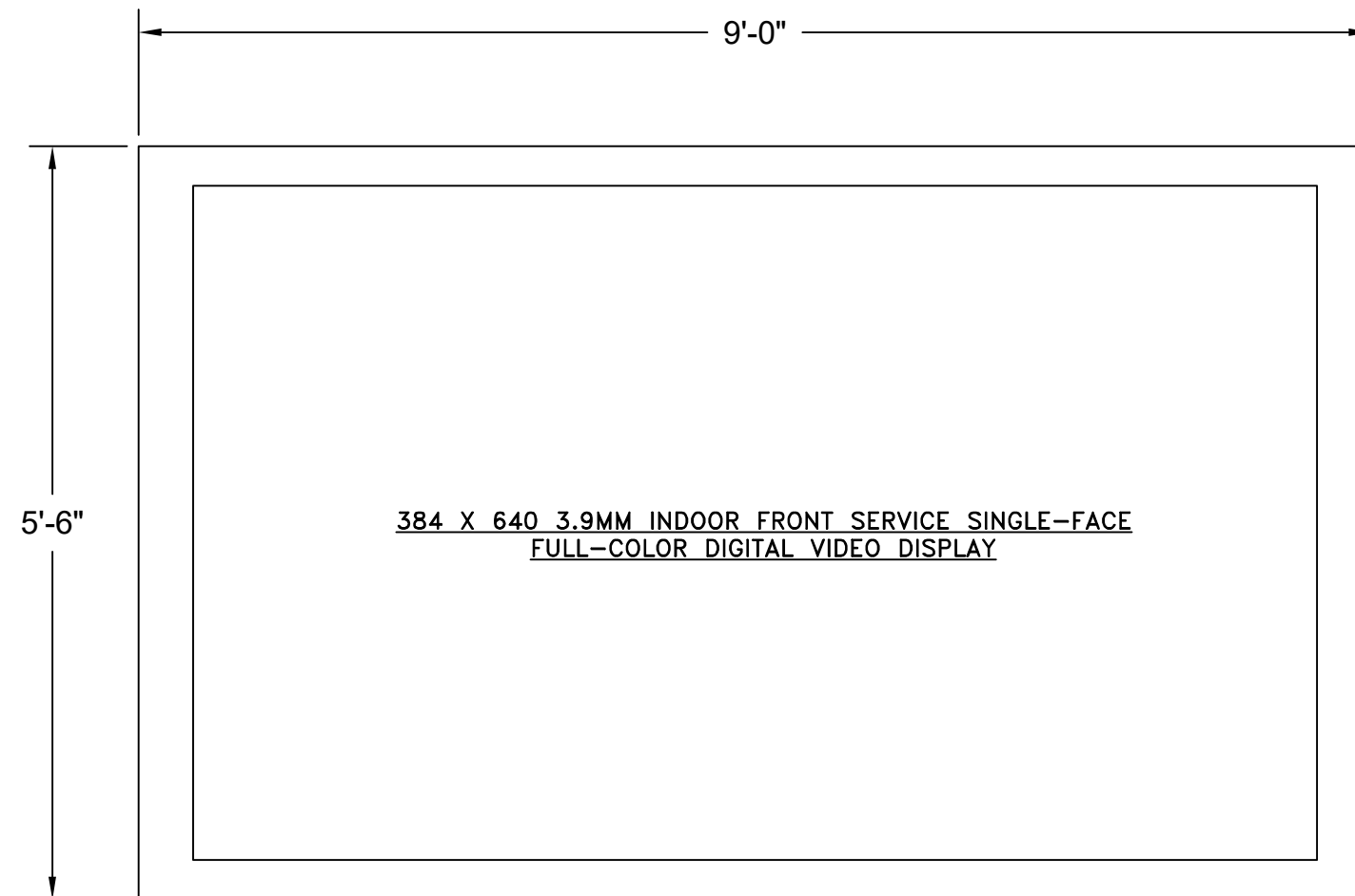
FACE VIEW SHOWN WITH 9'-0"L X 5'-6"H TRIM KIT, USING INDOOR FRAME
