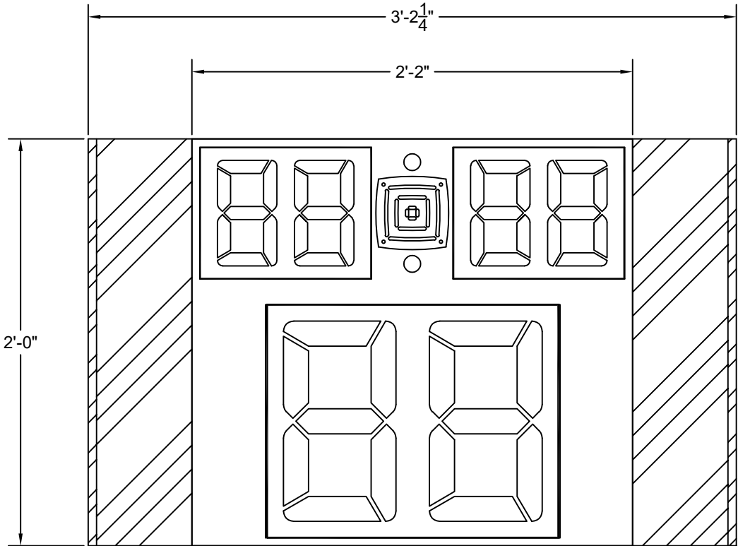
ST-1420-3S-4 LED BAR DIGIT INDOOR SHOT TIMER/GAME CLOCK SET FACE 1 SHOWN, OTHERS TYPICAL
