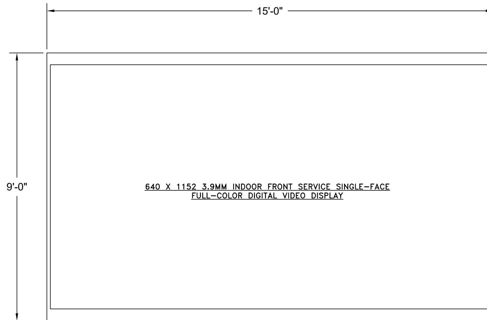
FACE VIEW SHOWN WITH 15'-0"L X 9'-0"H TRIM KIT. USING INDOOR FRAME
