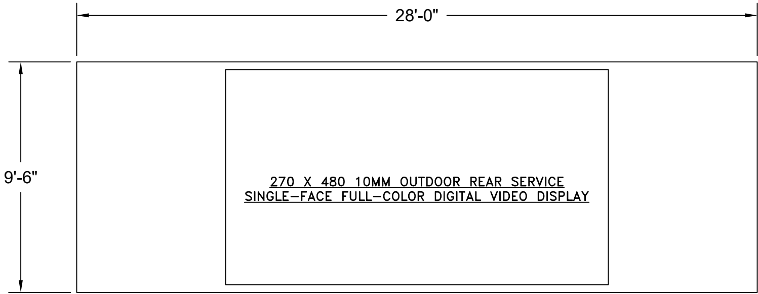
FACE VIEW SHOWN WITH 28'-0"L X 9'-6"H TRIM KIT, USING FRAME
