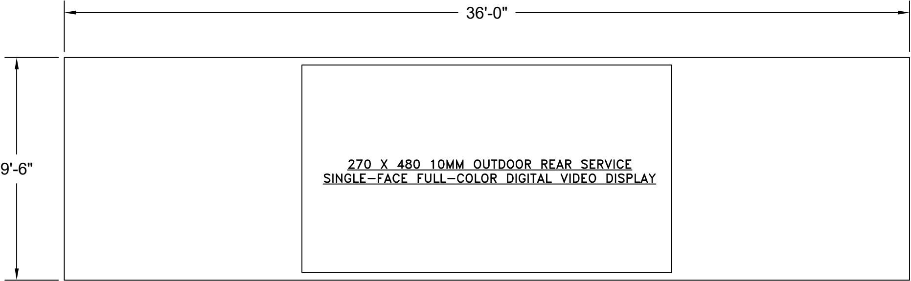
FACE VIEW SHOWN WITH 36'-0"L X 9'-6"H TRIM KIT, USING FRAME
