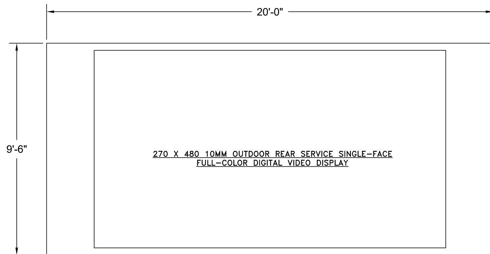
FACE VIEW SHOWN WITH 20'-0"L X 9'-6"H TRIM KIT, USING FRAME
