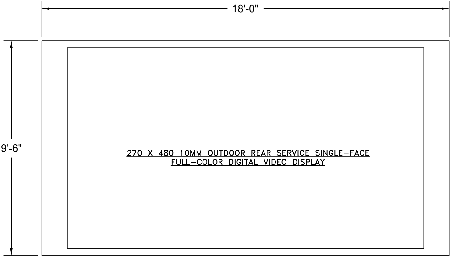
FACE VIEW SHOWN WITH 18'-0"L X 9'-6"H TRIM KIT, USING FRAME
