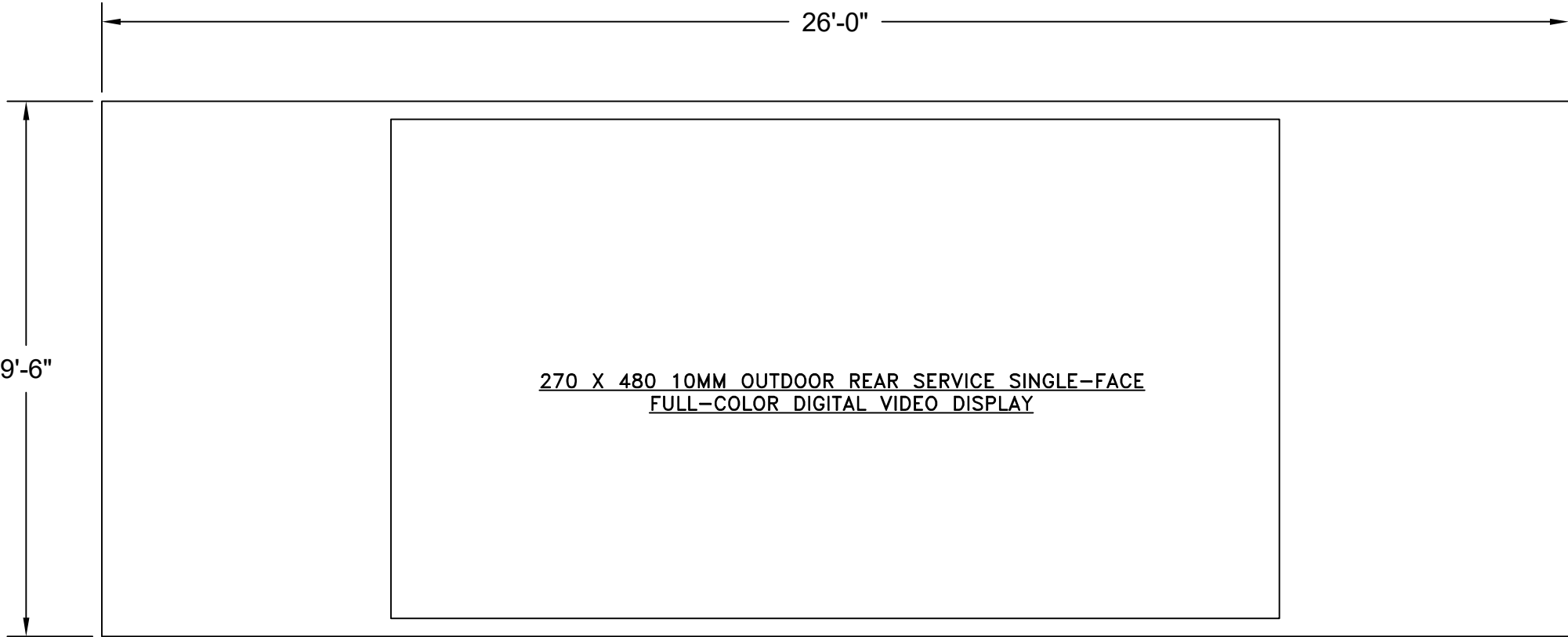
FACE VIEW SHOWN WITH 26'-0"L X 9'-6"H TRIM KIT, USING FRAME
