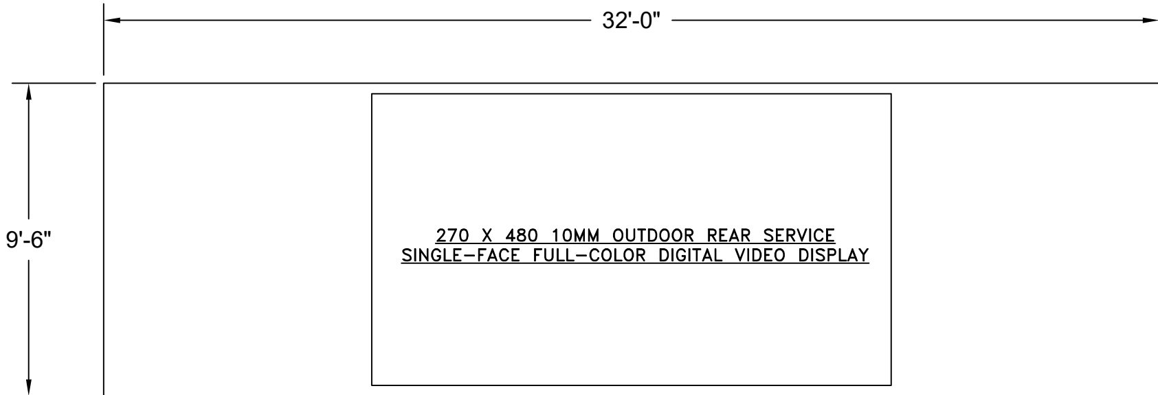
FACE VIEW SHOWN WITH 32'-0"L X 9'-6"H TRIM KIT, USING FRAME
