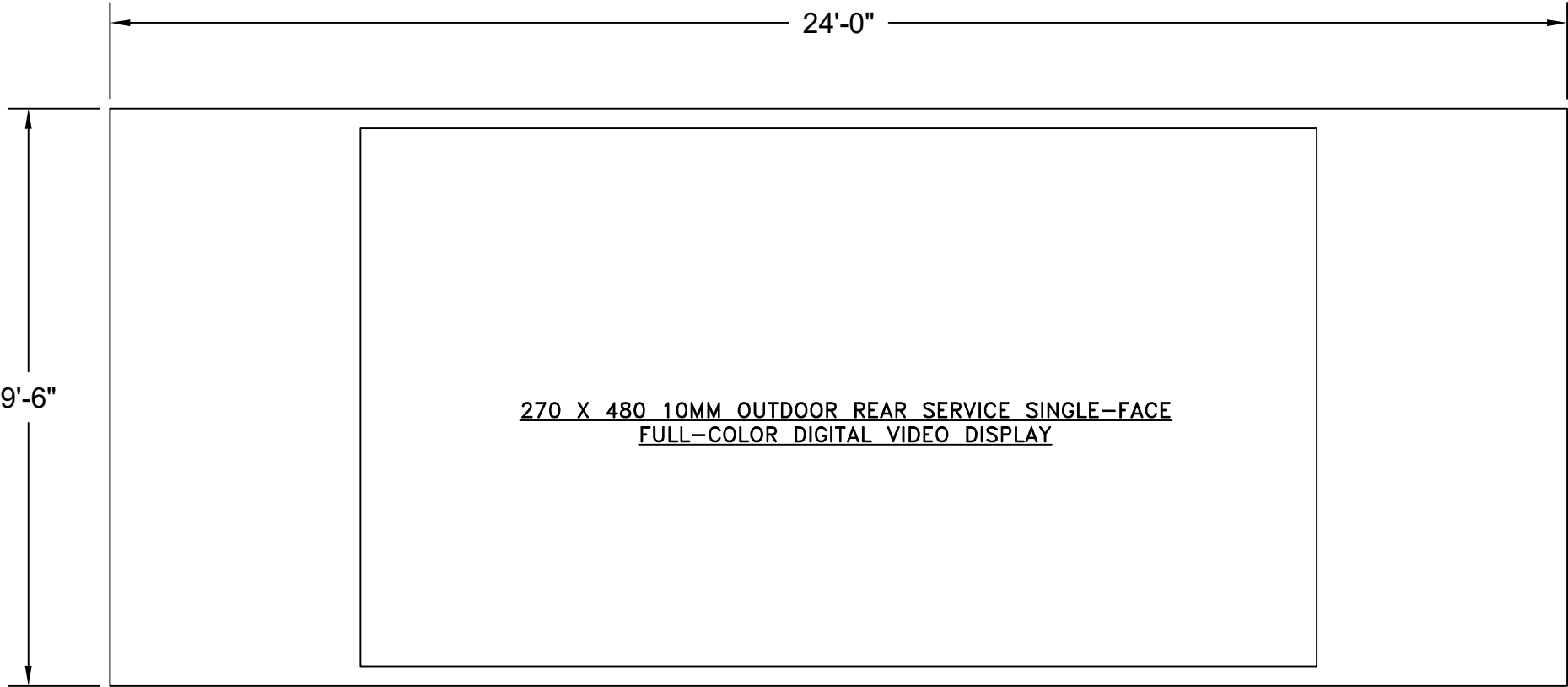
FACE VIEW SHOWN WITH 24'-0"L X 9'-6"H TRIM KIT, USING FRAME
