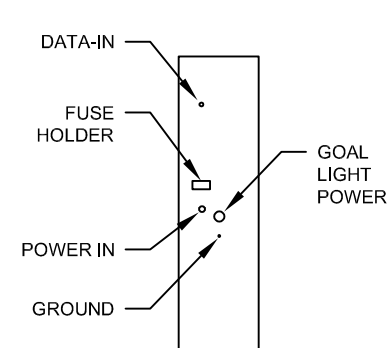
LEFT VIEW
