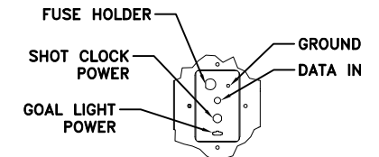
CONNECTION DETAIL
