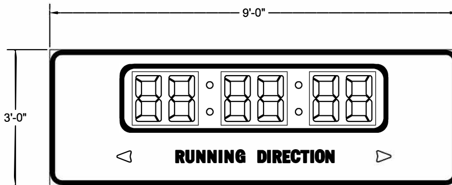
PC-1450-4 PACE CLOCK SCOREBOARD
