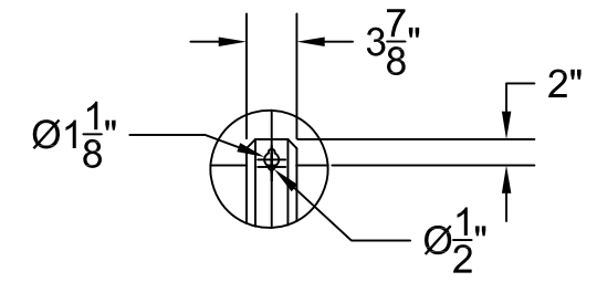
DETAIL A MOUNTING BRACKET
