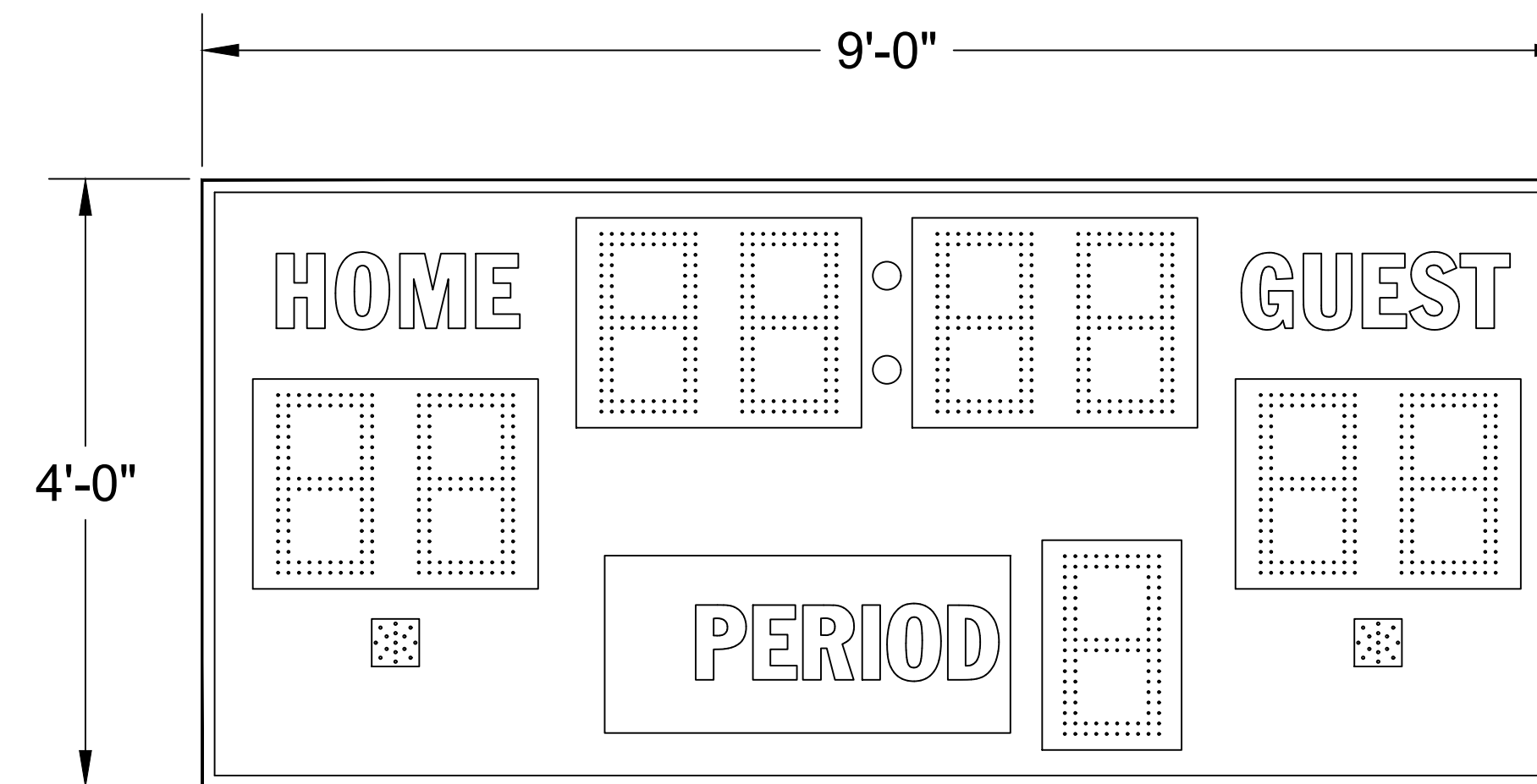
MP-8109-2 FOOTBALL/SOCCER ARRANGEMENT
