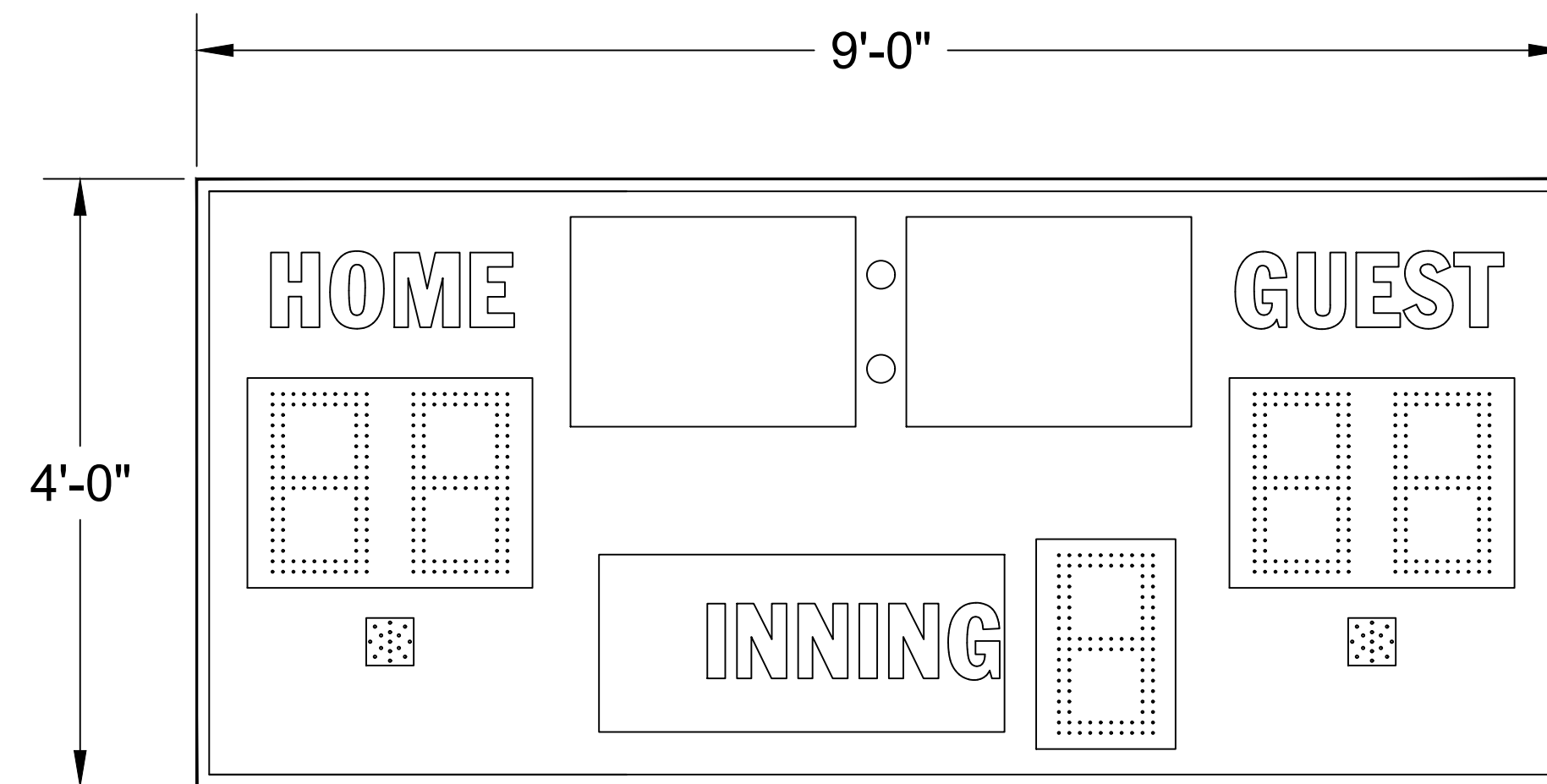
MP-8109-2 BASEBALL ARRANGEMENT
