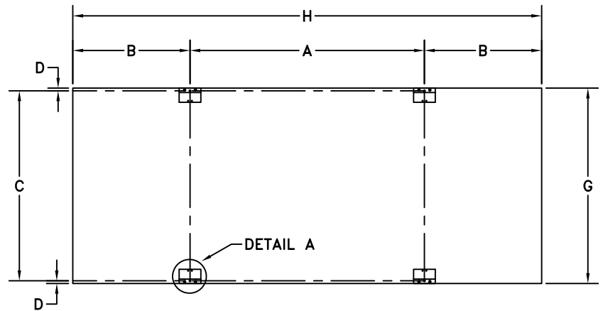
HANGER BRACKET DETAIL (BACK VIEW)
