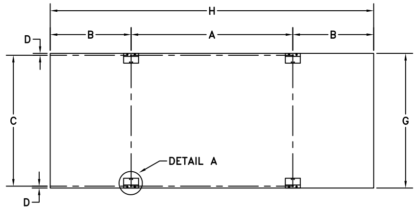
FB-8318-2 HANGER BRACKET DETAIL (BACK VIEW)
