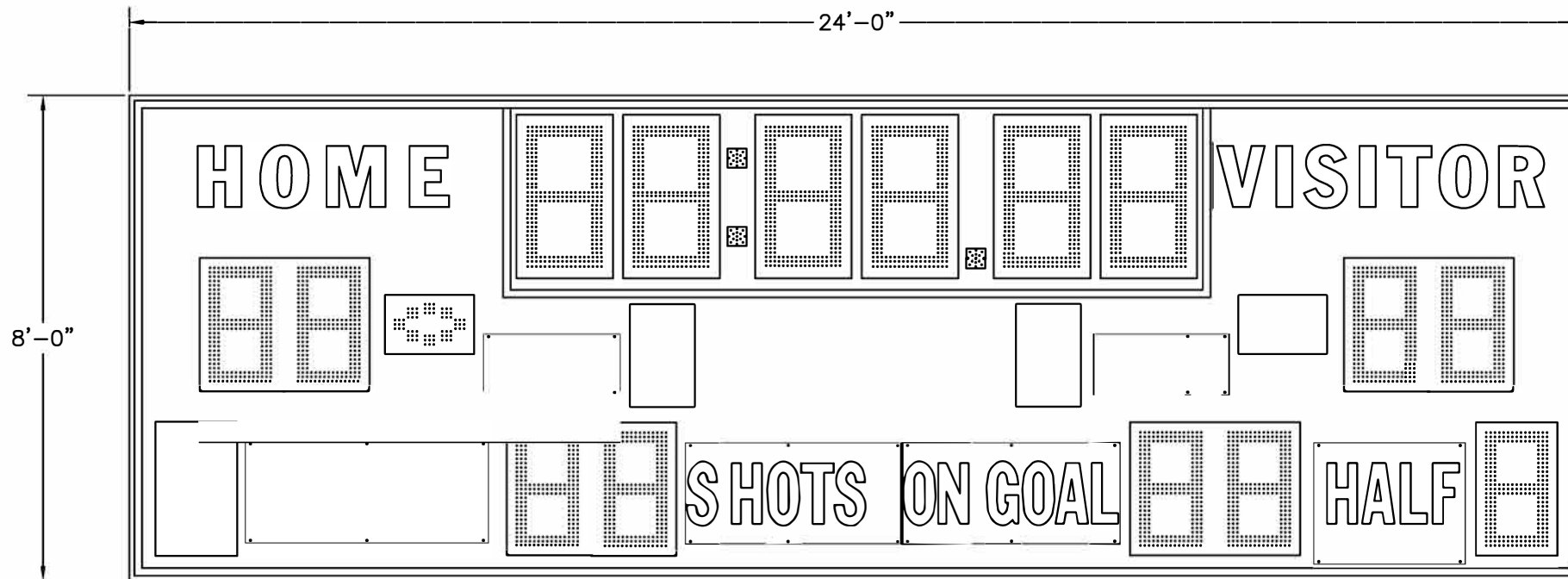
FB-8124-2 WITH TKH CLOCK SOCCER ARRANGEMENT
