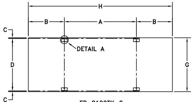
FB-8120TK-2 HANGER BRACKET DETAIL (BACK VIEW)
