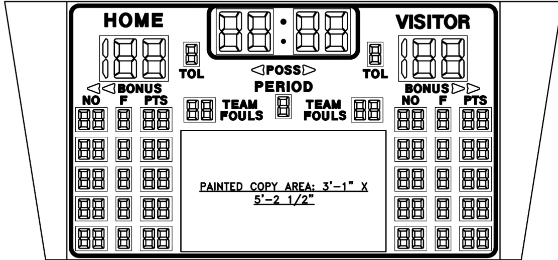
BB-1855A-4 FOUR-SIDED BASKETBALL SCOREBOARD FACE 1 OF 4 SHOWN - ALL OTHERS TYPICAL
