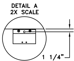
STANDARD "J" BRACKET 1/4" STEEL
