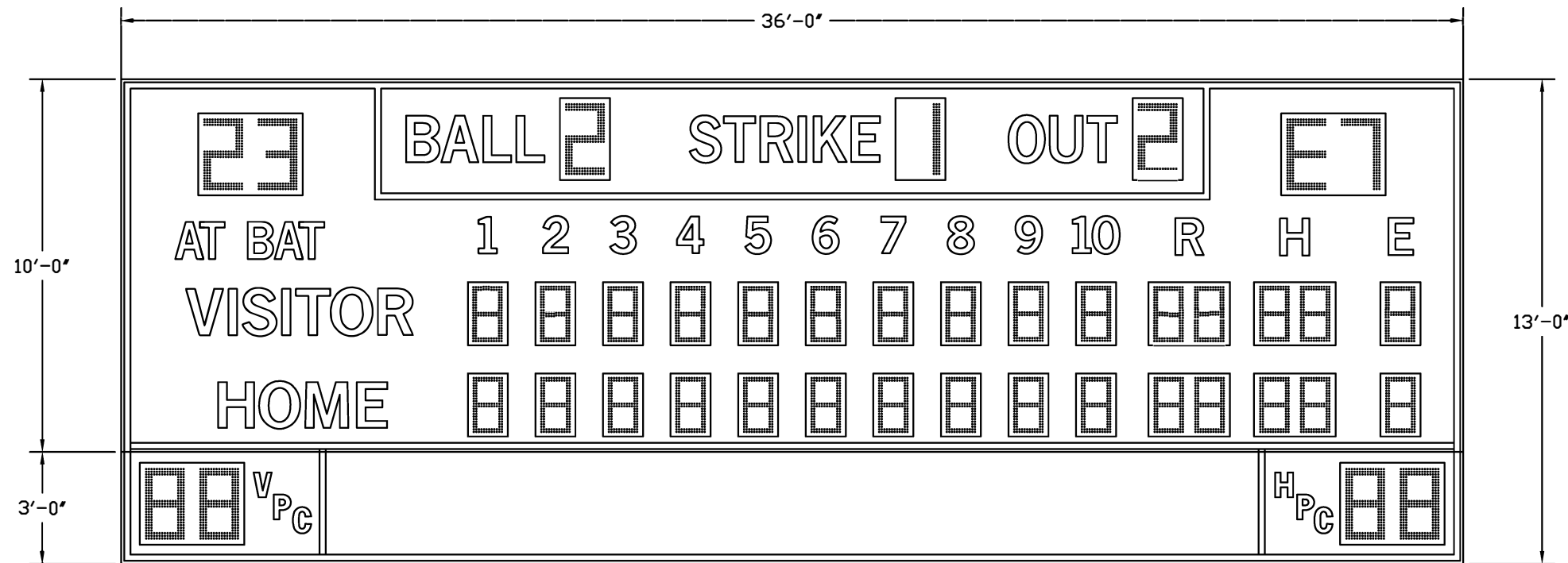
BA-7136PC-2 (24"H DIGITS MOVED TO THE ENDS OF PITCH COUNT SECTION, ADDED TRIM)
