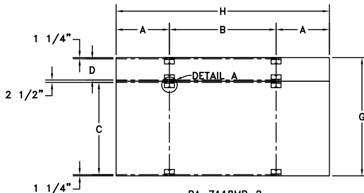
BA-7118MP-2 HANGER BRACKET DETAIL BACK VIEW
