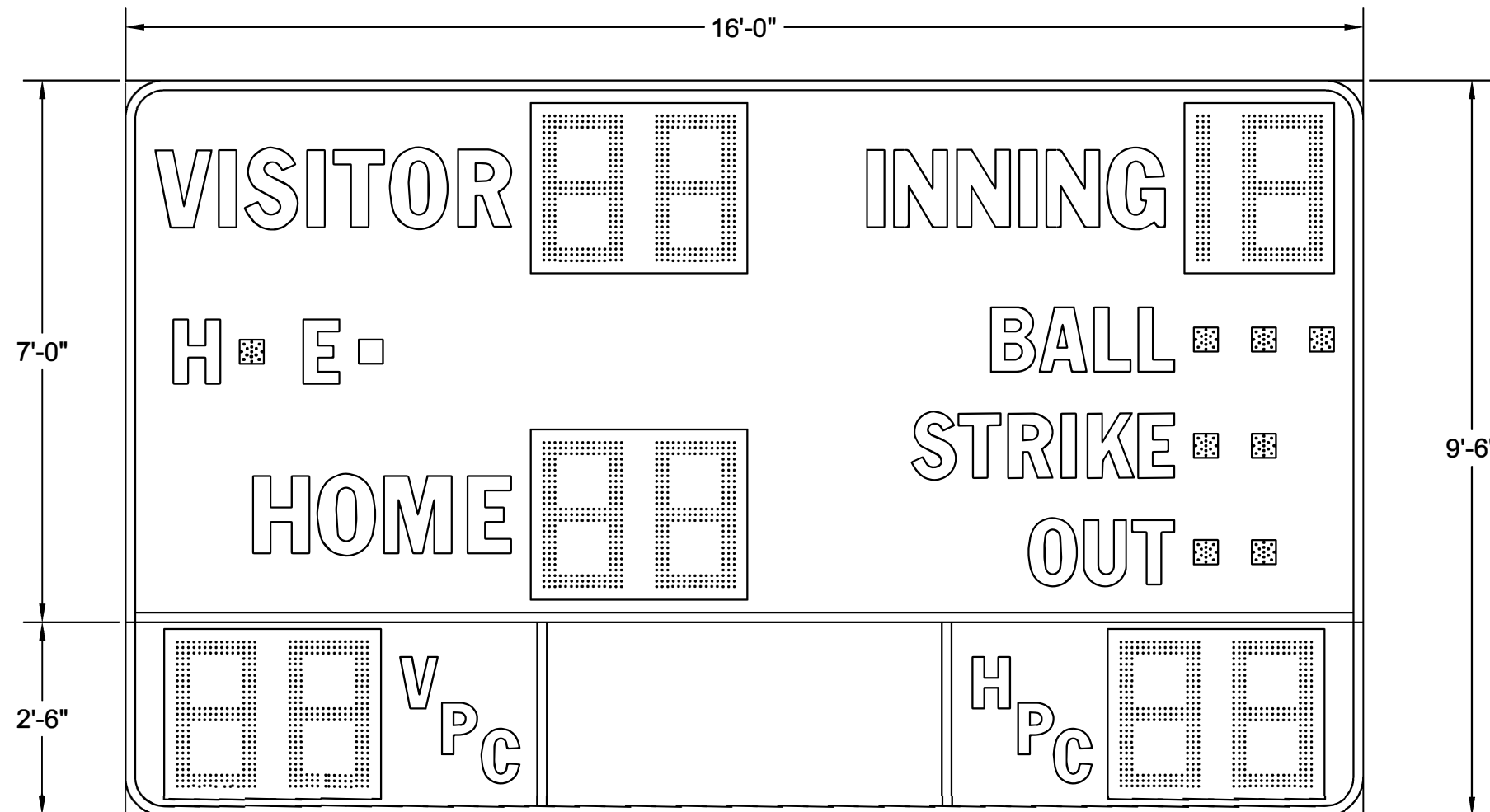
BA-7116PC-2 (24"H DIGITS MOVED TO THE ENDS OF PITCH COUNT SECTION, ADDED TRIM)
