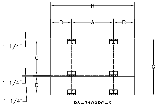
BA-7109PC-2 HANGER BRACKETS (BACK VIEW)
