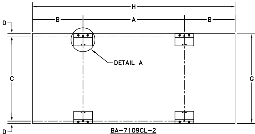
BA-7109CL-2 HANGER BRACKETS (BACK VIEW)
