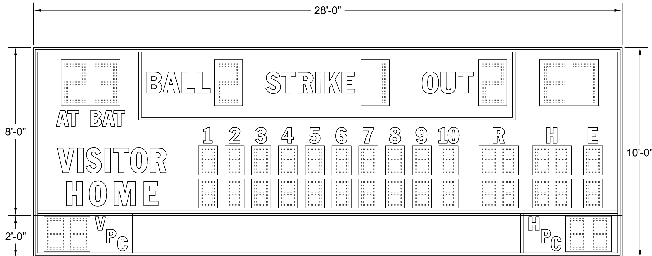
BA-7128PC-2 (18"H DIGITS MOVED TO THE ENDS OF PITCH COUNT SECTION, ADDED TRIM)
