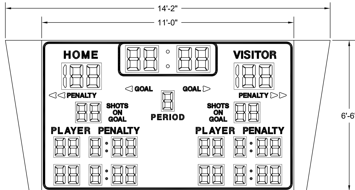
HK-1885-4 4-SIDED HOCKEY SCOREBOARD FACE 1 OF 4 SHOWN - ALL OTHERS TYPICAL
