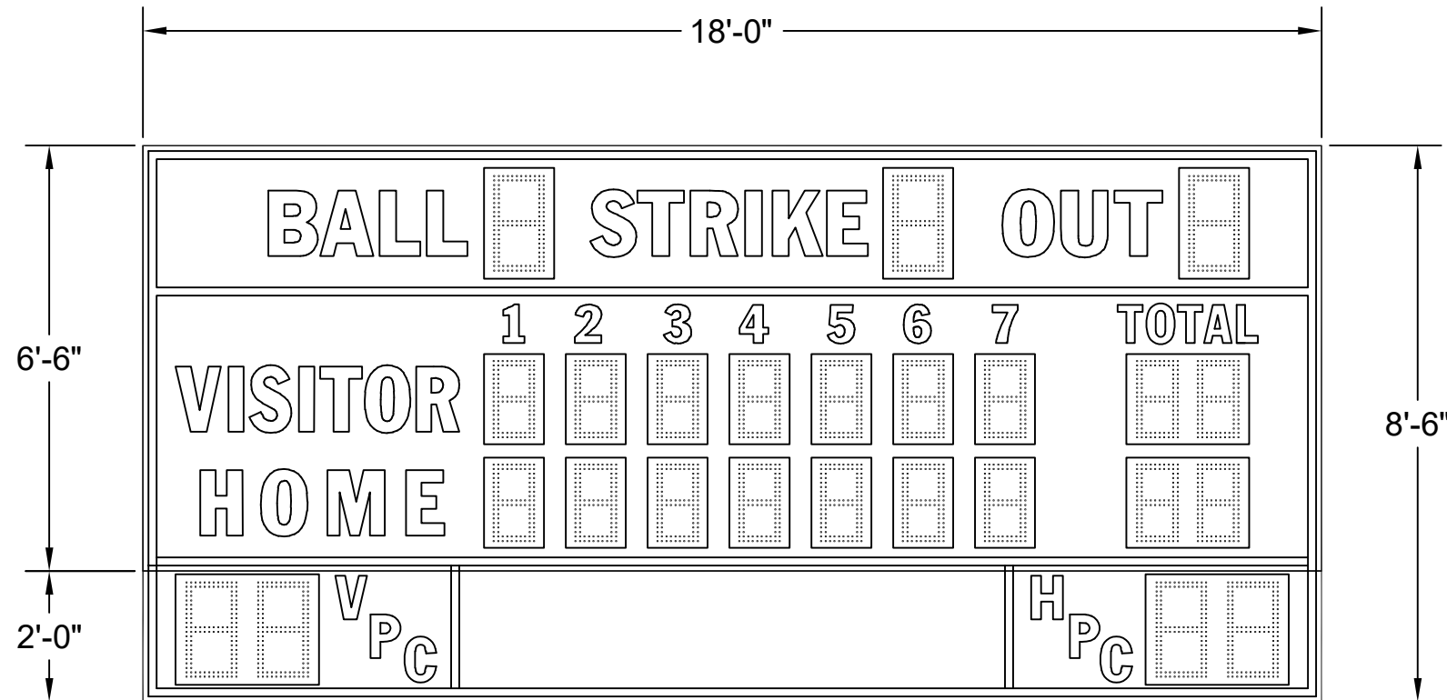
BA-7218PC-2 (18"H DIGITS MOVED TO THE ENDS OF PITCH COUNT SECTION, ADDED TRIM)
