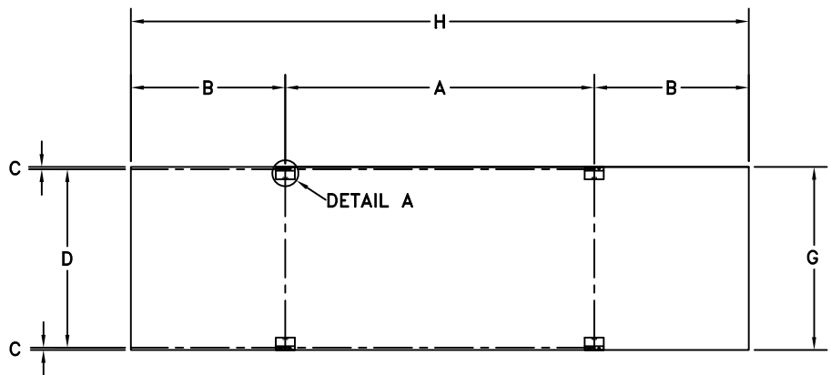
FB-8127-2 HANGER BRACKETS BACK VIEW
