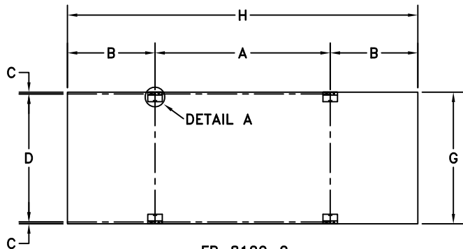
FB-8120-2 HANGER BRACKET DETAIL (BACK VIEW)
