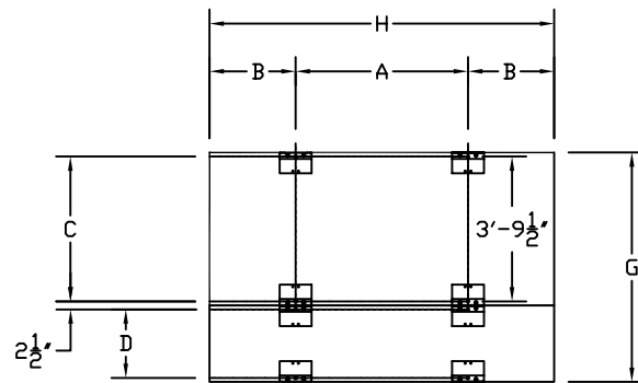
BA-7209-2 HANGER BRACKET DETAIL (BACK VIEW)
