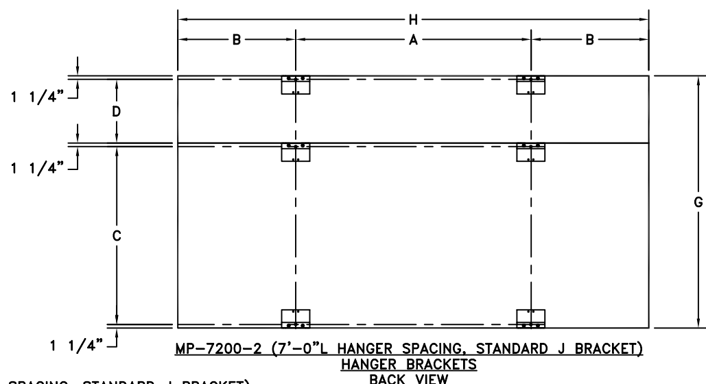
DIMENSIONS MP-7200-2 (7'-0" L HANGER SPACING, STANDARD J BRACKET)
