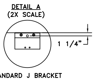
DIMENSIONS MP-7200-2 (7'-0" L HANGER SPACING, STANDARD J BRACKET)
