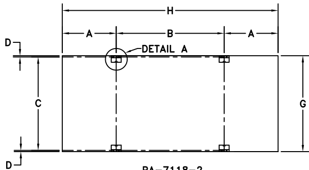
BA-7118-2 HANGER BRACKET DETAIL BACK VIEW
