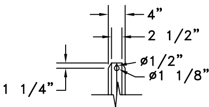
DETAIL A MOUNTING BRACKET SCALE 2X
